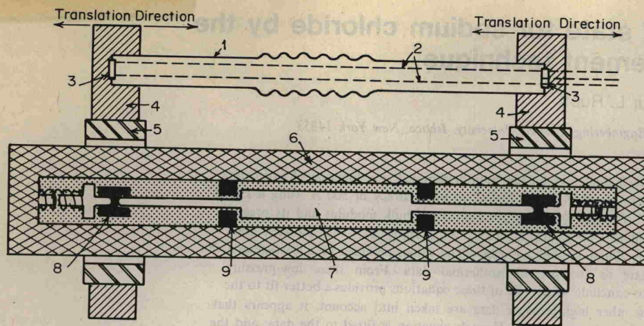
FIG. 1. Schematic of length-measurements system: (a) laser path vacuum bellows; (2) laser beam; (3) interferometer mirrors; (4) coupling plates; (5) LVDT's; (6) pressure vessel; (7) specimen; (8) magnetic cores; (9) ball bushings.
